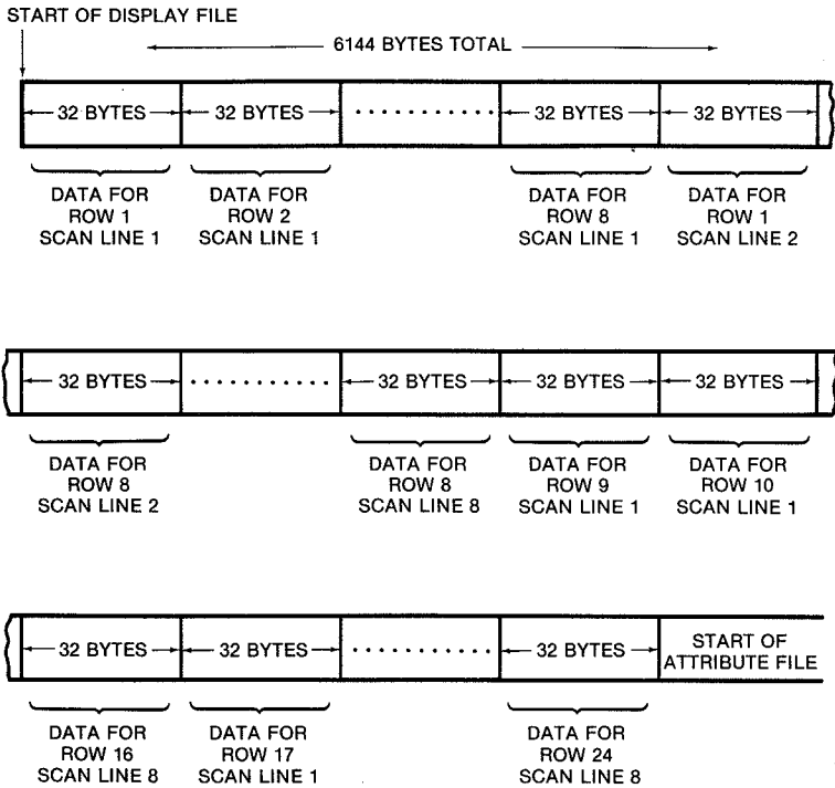
Fig. 8-5. Display file organization. (Courtesy Timex Computer Corp.)
